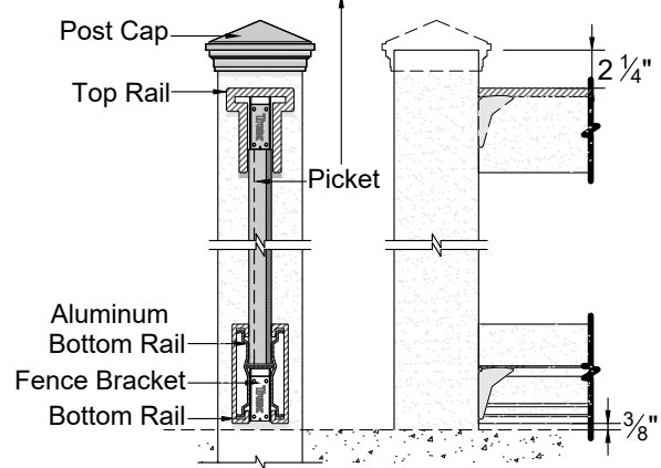
CUT VIEWS
