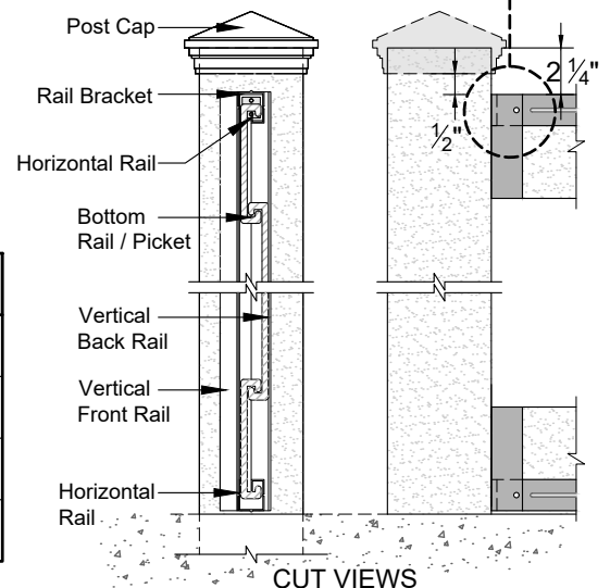
CUT VIEWS
